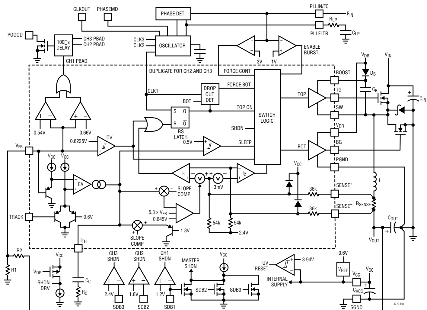
Figure 1. Functional Diagram
